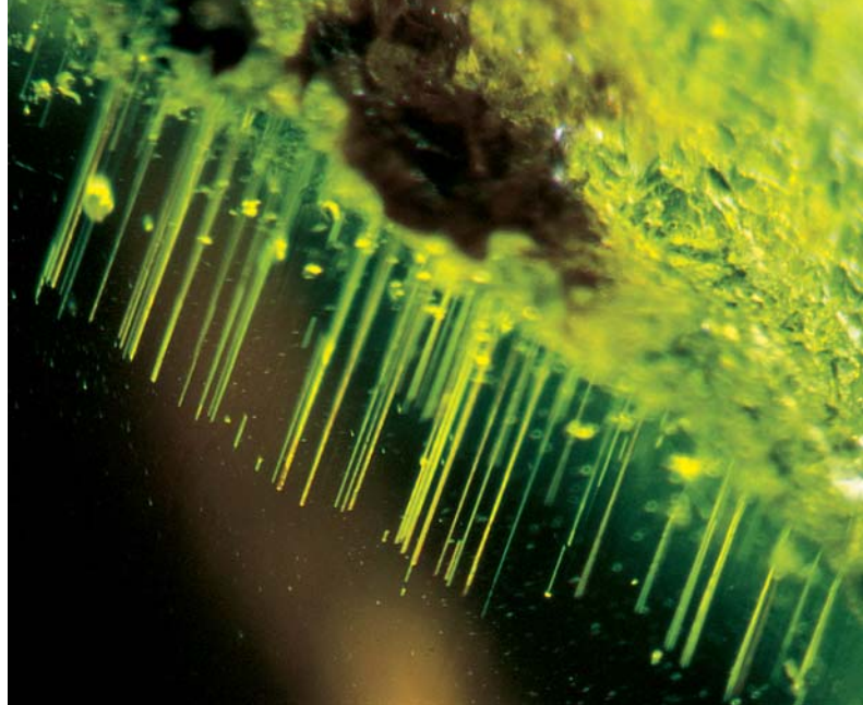
Figure 6. Some of the growth tubes in the green rind of this 12.02 ct multicolored tourmaline nodule are partially filled with an orange material. Photomicrograph by John I. Koivula; magnified 20 \times .
